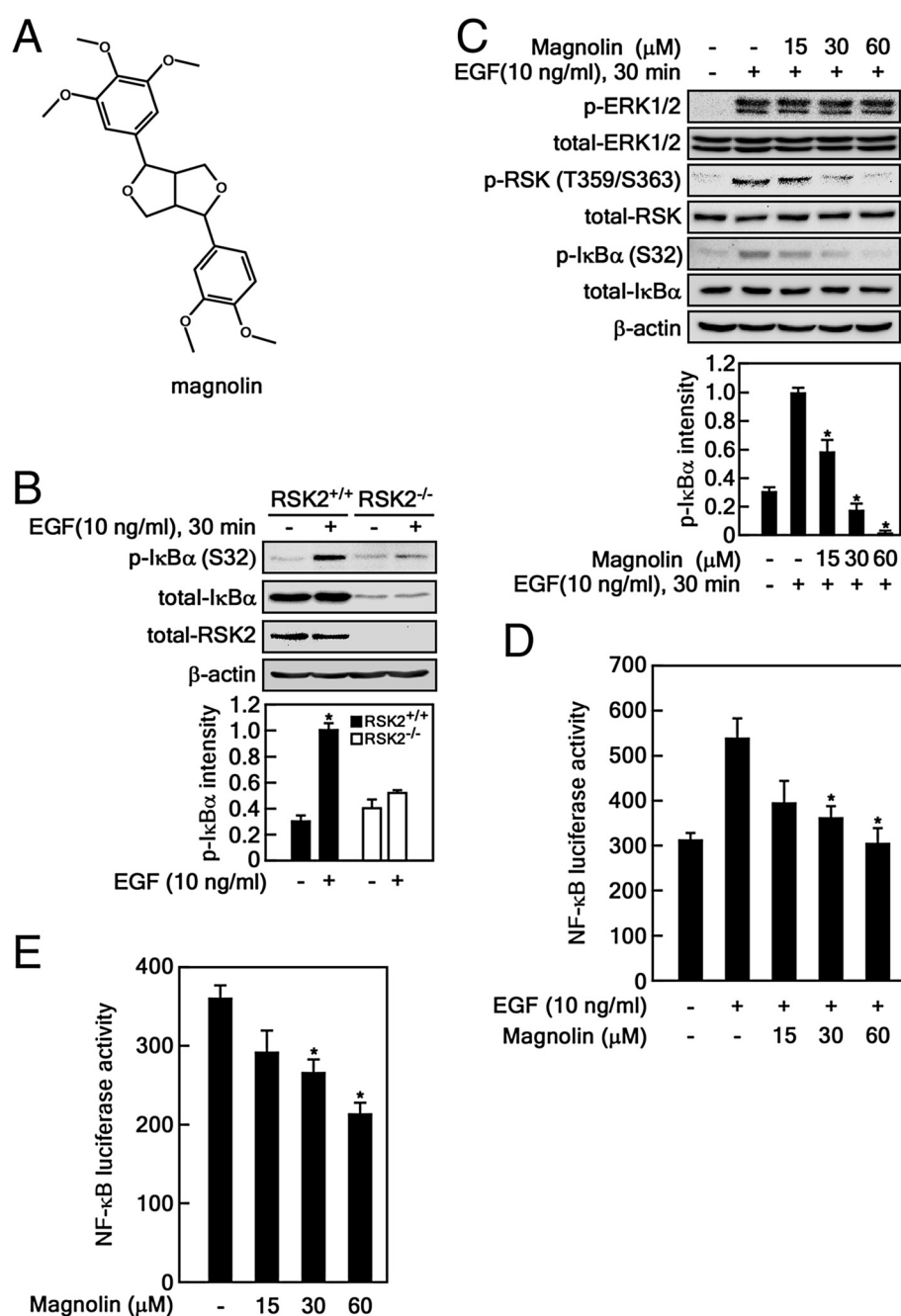
Fig. 1 Magnolin inhibits NF-κB transactivation activity. a Chemical structure of magnolin. b RSK2 mediates IκBα phosphorylation at Ser32. RSK2 +/+ and RSK2 -/- MEFs were used to visualize the phosphorylation of IκBα induced by EGF stimulation using the specific antibodies as indicated. c Magnolin inhibits EGF-induced IκBα phosphorylation at Ser32. JB6 Cl41 ( 1 \times 10^6 ) cells were seeded, starved, and treated with magnolin in the presence or absence of EGF. The specific protein levels were visualized by Western blotting using the specific antibodies as indicated. b-c β-actin was used as an internal control to verify equal protein loading. d-e Magnolin inhibits EGF-induced NF-κB transactivation activity. JB6 Cl41 cells stably expressing NF-κB luciferase reporter plasmid were seeded, cultured, starved, and stimulated with EGF and the indicated doses of magnolin ( d ), or treated with the indicated doses of magnolin under normal culture conditions for 24 h ( e ). Firefly luciferase activity was measured as described in "Materials and Methods". b-e Data are presented as the mean \pm S.D. of values from triplicate experiments, and statistical significance was determined using the Student's t -test (*, p < 0.05 )
