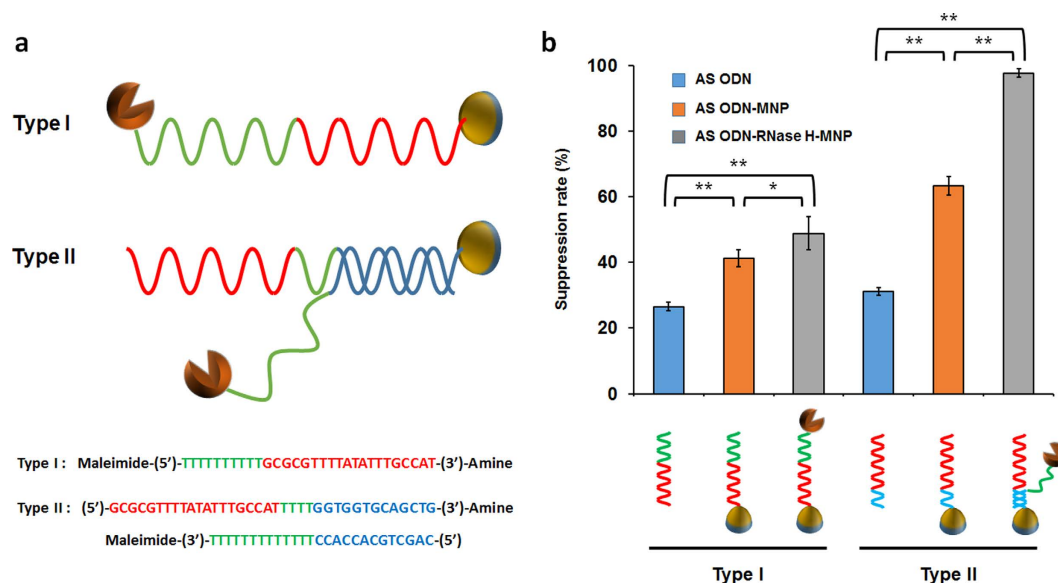
Figure 4. Design and comparison of molecular nanodevices consisting of ASODN, RNase H and magnetic nanoparticles. (a) Schematic of the two designed MNP conjugates with ASODN and RNase H. Red letters, ASODN regions; green letters, linker regions; blue letters, complementary regions. (b) Comparison of suppression rates of the two designed nanodevices during cell-free protein synthesis of sfGFP. Final concentration of ASODN was set at 2 μM and approximately same concentrations of RNase H was conjugated on MNPs. Error bars in the graph indicate standard deviations from three independent reaction samples. *p-value < 0.05. **p-value < 0.01.
