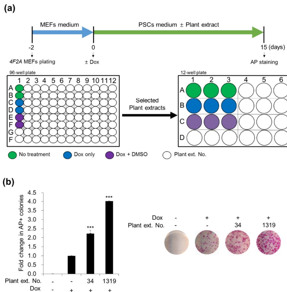
Figure 1. Screening and identification of plant extracts No. 34 and No. 1319 from Camellia japonica (CJ) that promote mouse embryonic fibroblasts (MEF) reprogramming. (a) Schematic experimental procedure of high-throughput screening. The 4F2A MEFs were seeded at 7.5 \times 10^3 cells per well in 96-well plates. After 2 days, cells were treated with or without plant extracts and cultured in doxycycline (dox) to activate Oct-4, Sox-2, Klf-4, and c-Myc (OSKM) expression. The number of alkaline phosphatase (AP)+ colonies on day 15 post-treatment was used as a measure of the reprogramming efficiency. (b) Identification of CJ extracts No. 34 and No. 1319 that enhance reprogramming. The relative fold changes of AP+ colonies compared with dimethyl sulfoxide (DMSO)-treated control and cultured in dox were presented as the mean + standard error of the mean (SEM) of three independent experiments. Statistical significance was determined using Student's t -test (** p -value < 0.001). Representative images of AP+ colonies per well were presented in the right panel.
