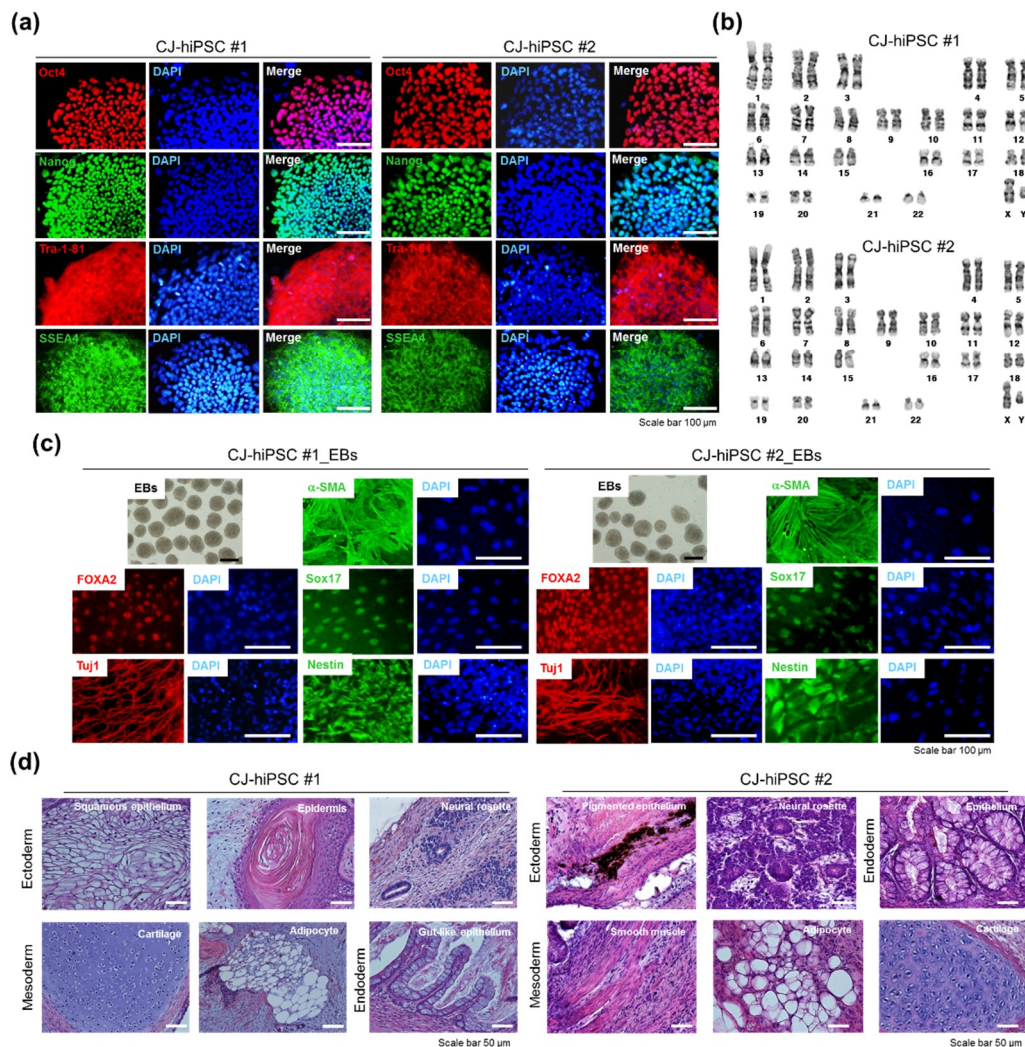
Figure 4. Characterization of CJ -extract-induced hiPSC clones ( CJ -hiPSCs). (a) Representative images of CJ -hiPSCs #1 and #2 depicting typical morphology and expression of pluripotency markers, including Oct4, Nanog, SSEA-4, and Tra-1-81. Scale bars, 100 \mu m. (b) Normal karyotype of CJ -hiPSCs #1 and #2. (c) In vitro embryoid body (EB) differentiation of CJ -hiPSCs #1 and #2. Bright field images of representative EBs and immunocytochemical analysis of mesoderm ( \alpha -SMA), endoderm (FOXA2 and Sox17), and ectoderm (Tuj1 and Nestin) markers in differentiated cells. The cells were co-stained with DAPI (blue). Scale bars, 100 \mu m. (d) Histological analysis of teratomas derived from CJ -hiPSCs #1 and #2. Ectoderm was represented by neural tissue and epidermis. Mesoderm was represented by cartilage, adipocyte, and muscle. Endoderm was represented by epithelium. Scale bars, 50 \mu m.
